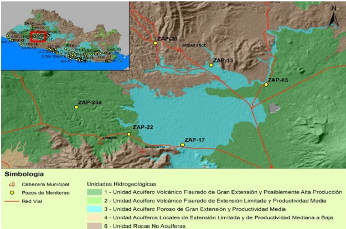
Figure 6. Map of groundwater monitoring network - Zapotitán
