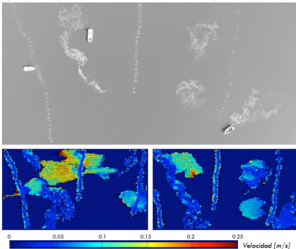
Figure 3. Monitoring the effectiveness of aeration diffusers in the San Roque Reservoir - LSPIV
