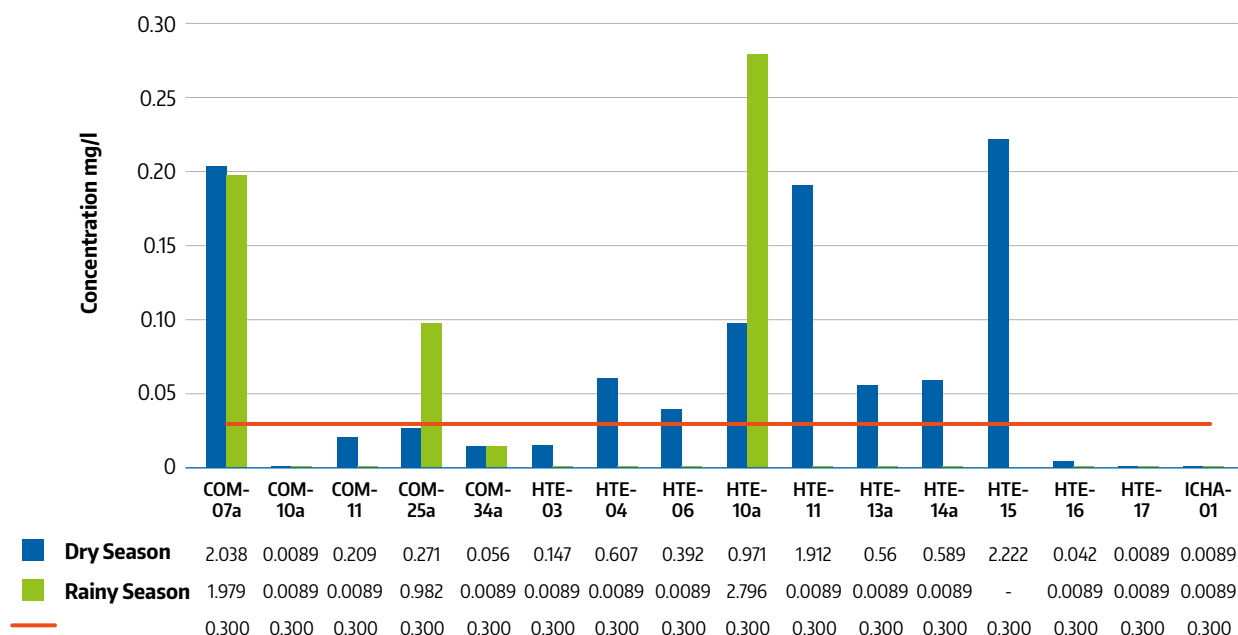
Figure 9. Iron concentration
