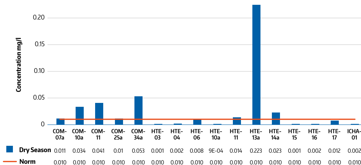
Figure 8. Arsenic concentrations
