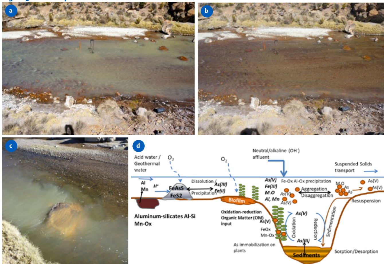
Figure 3. Arsenic dynamics in the Lluta river basin
