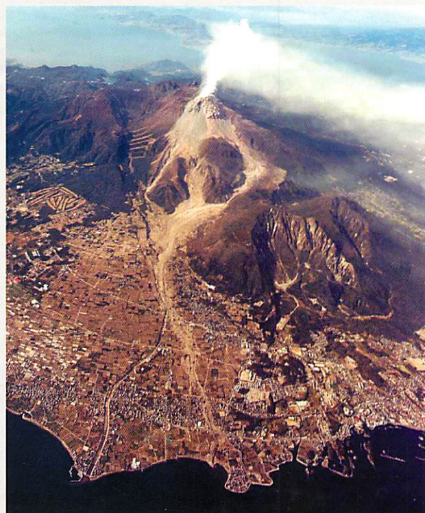
The gigantic Mayuyama Landslide on Mount Unzen in Japan in 1992; the 200 million m 3 of debris and induced tsunami killed 16,000 people
